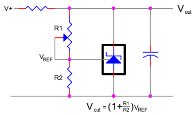
Figure 1. Shunt Regulator
